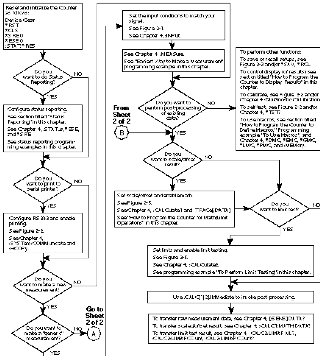
Figure 3-11. SCPI Programming Flowchart (Sheet 1 of 2)
