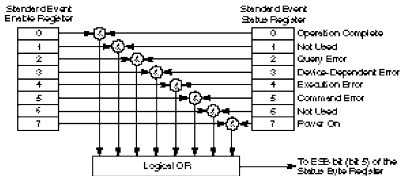
Figure 3-8. Standard Event Status Reporting
